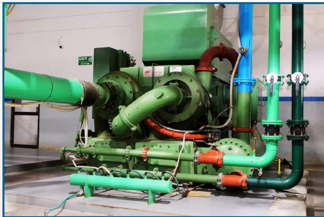
INGERSOLL RAND Compressor TA 6000 (670 KW)
